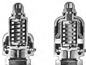
Figs. 3222. Star Improved Pop Safety Valve.
